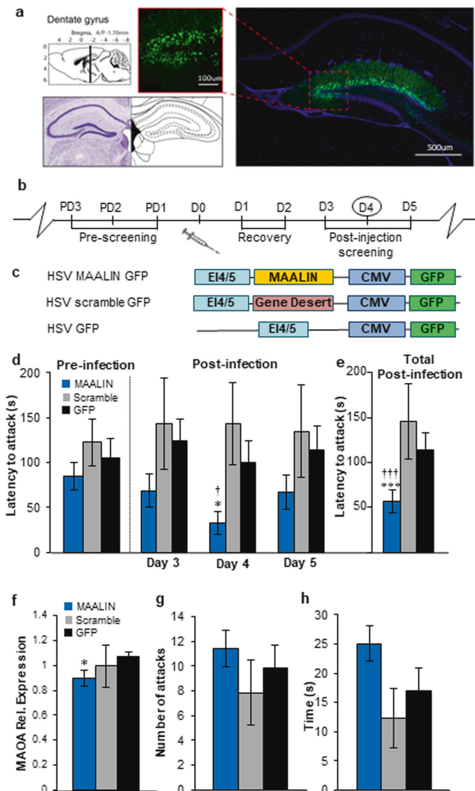
Fig. 5 Behavioural and functional impact of in vivo MAALIN overexpression.
